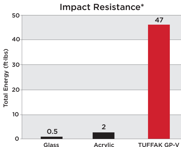
*Instrumented Impact per ASTM D 3763, sample thickness 0.125" nominal
